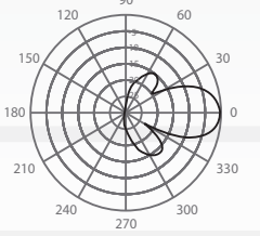
RF Patterns Horizontal Cut, typ.
